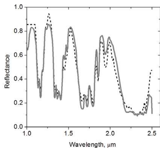
Fig. 2. Comparison between the measured spectrum of Makemake (dashed black line) and model that uses large ( \sim 0.3 \text{ mm} ) and small ( \sim 1 \mu\text{m} ) methane ice in a 70:30 mix (solid gray line).
