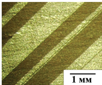
Fig. 1. Microphotograph of a typical structure of copper samples.
