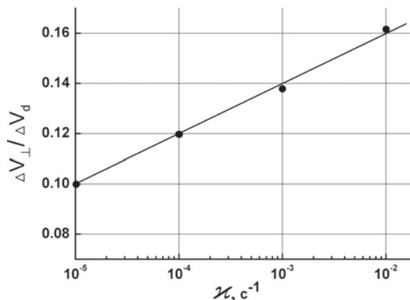
Fig.2. Relative portion of full misfit ( \Delta V_{\perp} / \Delta V_d ) versus cooling constant \alpha in KCl single crystals cooled from melting temperature T_m to room value T_{room} .
