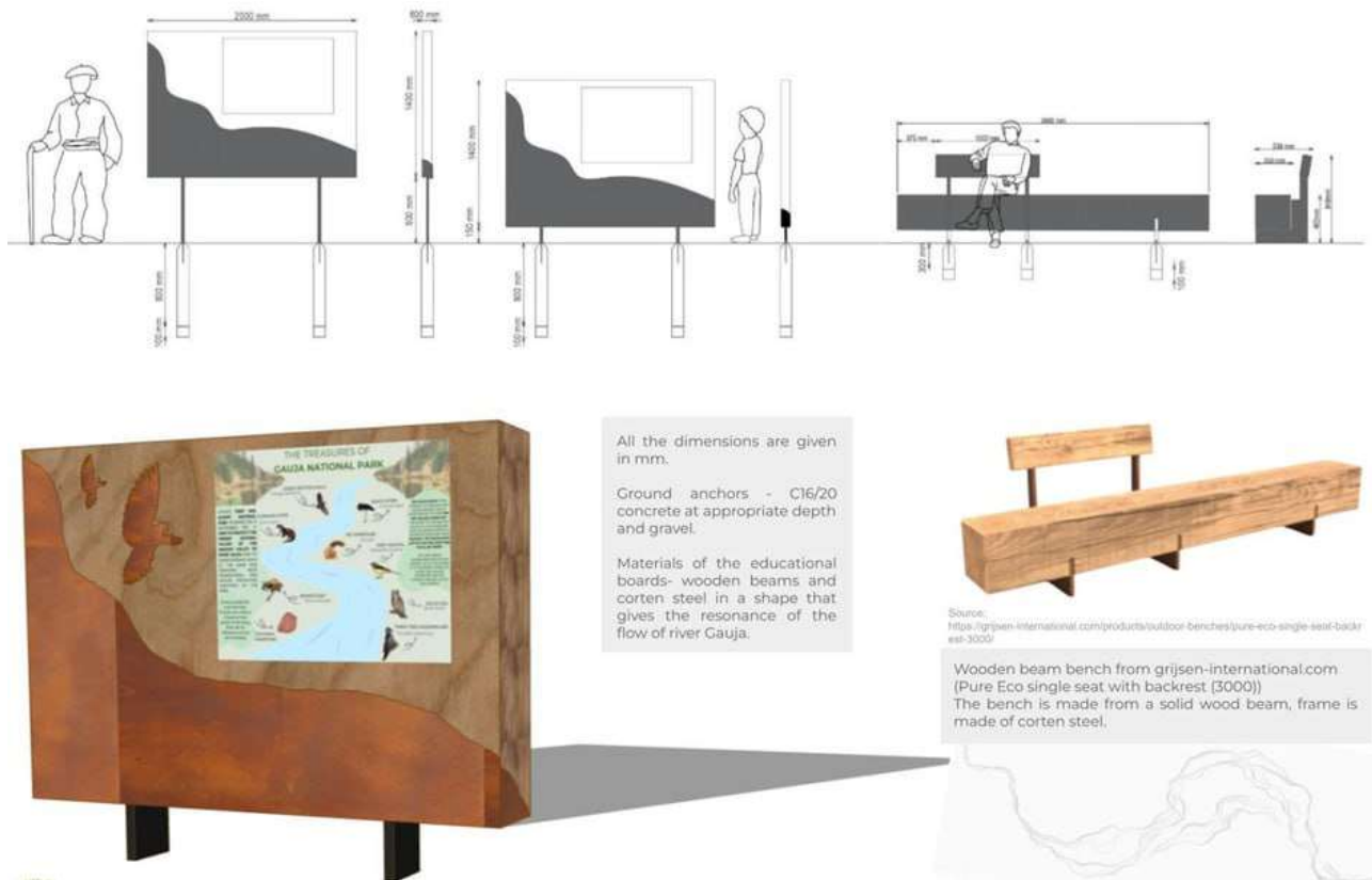
Fig. 3 – Design of the educational board and bench [12]
