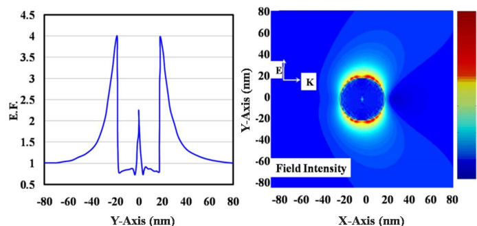
Figure 3. Electric field pattern of a 20 nm radius sphere (K||X, E||Y) on the right, and on the left field enhancement around a nano-sphere along the Y-axis.
