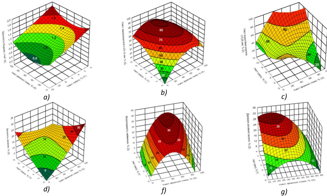
a) bulk of density; b) the contents of macroaggregates of 0,25-10 mm; c) the contents of waterproof aggregates > 0,25 mm;) d) humidity steady wilting of plants; f) the least moisture capacity; g) a range of an active moisture
