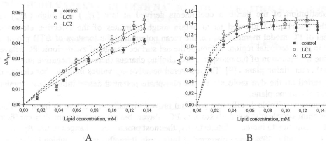
Fig. 3. Absorbance changes of the protonated BTB form as a function of lipid concentration at ionic strengths 5 mM (A) and 2 M (B). Drug concentration was 8 \mu M (LC1) or 6 \mu M (LC2). Dash lines represent theoretical curves calculated from Eq. 12
