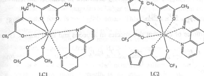
Fig. 1. Structure of lanthanide complexes.
